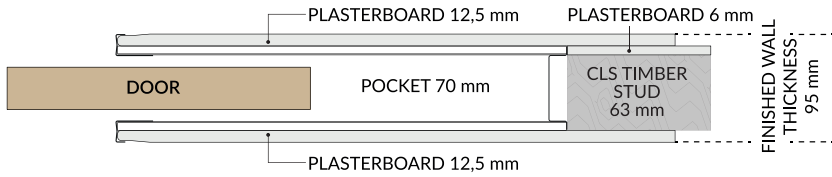
Pocket 70mm - Timber Stud 63mm CLS - Finished wall thickness 95mm
