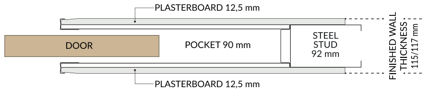
Pocket 90mm - Steel Stud 92mm - Finished wall thickness 115/117mm
