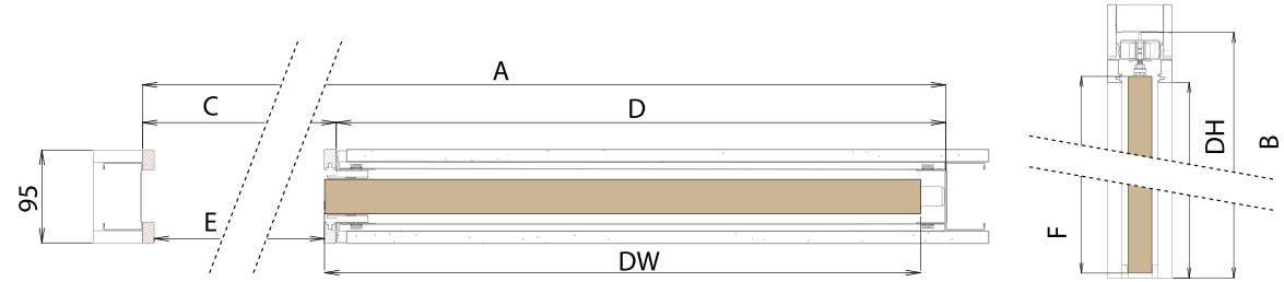
Pocket 70mm - Timber Stud 63mm CLS - Finished wall thickness 95mm
