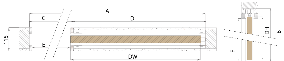
Pocket 90mm - Timber Stud 89mm CLS - Finished wall thickness 115mm
