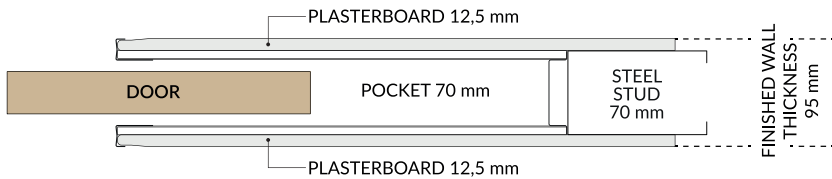
Pocket 70mm - Steel Stud 70mm - Finished wall thickness 95mm
